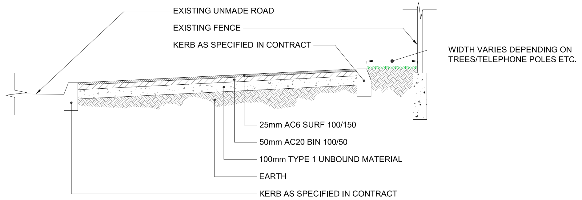
TYPICAL SECTION THROUGH PATH SCALE 1:25
